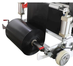
Unwinder with magnetic brake and air shaft
